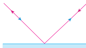
图4.2-6 光路可逆
